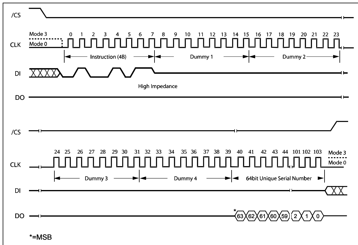
Figure 29. Read Unique ID Number Instruction Sequence Diagram
